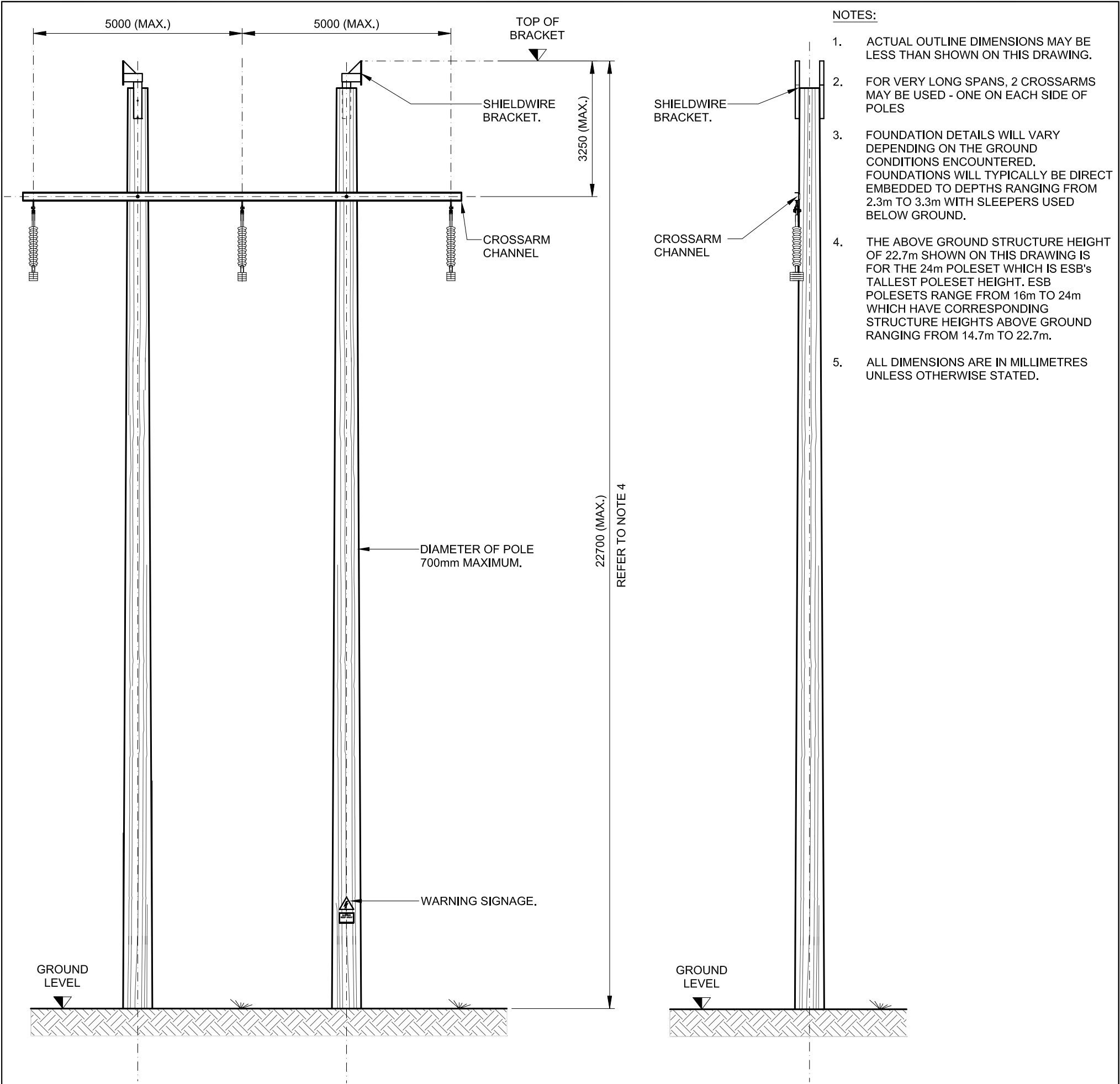
TYPICAL FRONT ELEVATION
